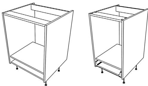
BUILT UNDER OVEN HOUSING Fixed fascia / working drawer
