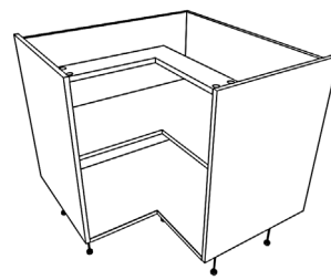
FULL HEIGHT 900 CORNER L-SHAPE BASE UNIT 330 x 330 front cut outs 4 x 170 degree hinges
