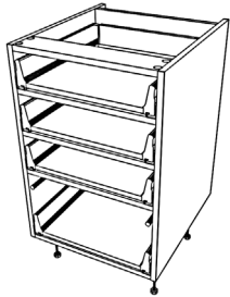
4 DRAWER BASE UNIT 3 x 140 drawers, 1 x 283 drawer
