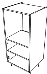
CONTINENTAL DOUBLE OVEN HOUSING 900 appliance. To take 1 door Height 1035 - 1335
