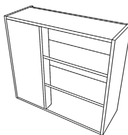
MEDIUM STANDARD CORNER WALL UNIT with a 300 blanking panel
